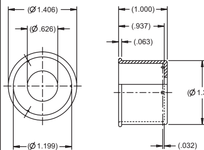
OTTO P/N C300302
